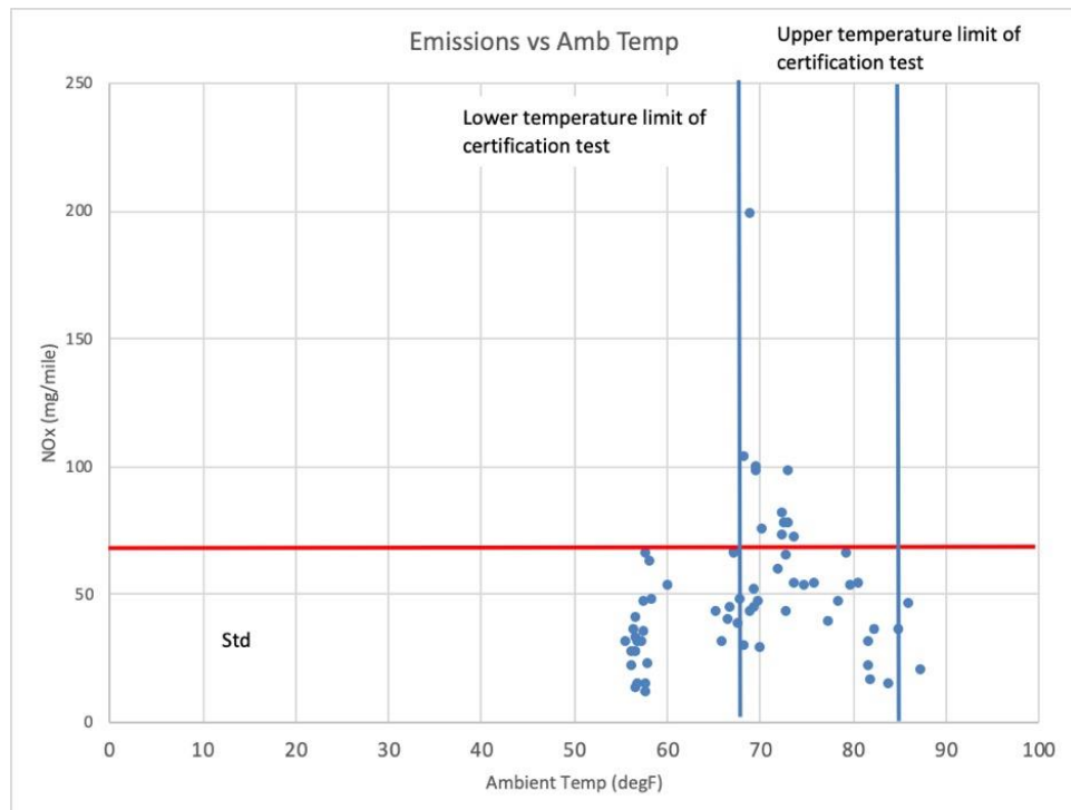
Figure 15: NOx emissions as a function of ambient temperature in highway driving conditions for 2011 335 Diesel B. Certification limit shown in red.
