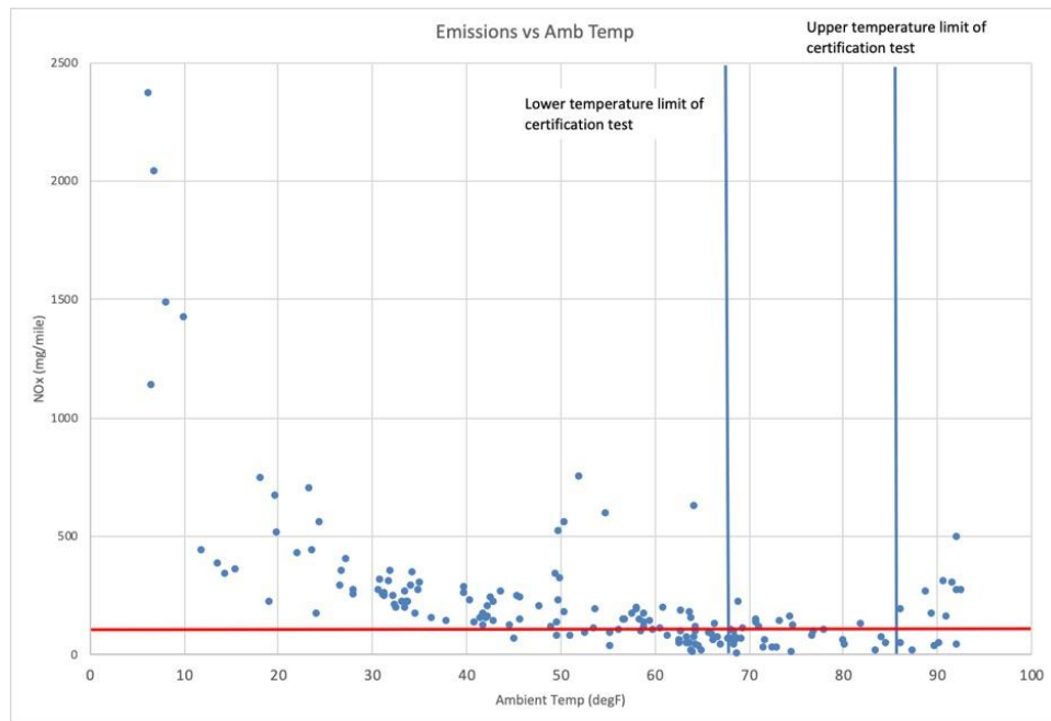
Figure 5: NOx emissions as a function of ambient temperature in highway driving conditions for 2012 X5 Diesel A. Certification limit shown in red.
