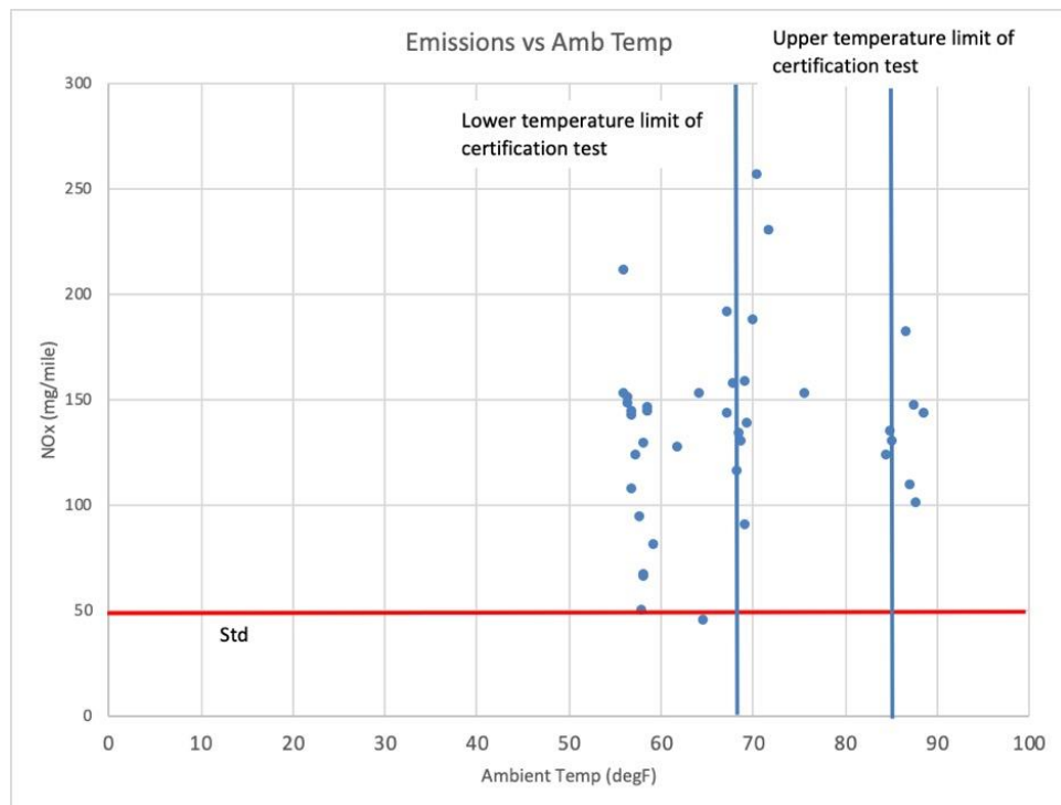
Figure 10: NOx emissions as a function of ambient temperature in city driving conditions for 2011 335 Diesel A. Certification limit shown in red.
